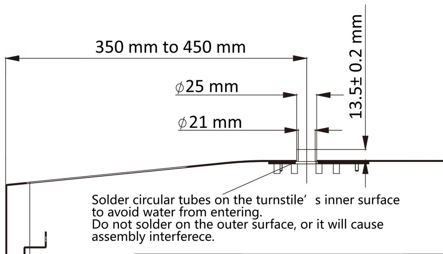
Figure 3-2 Solder Tubes
