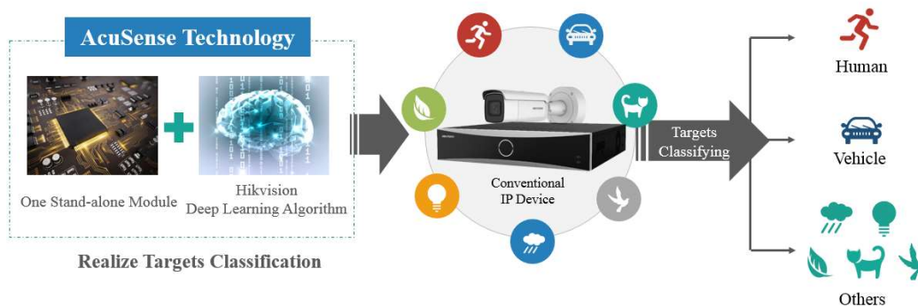
Figure 2 Target classification
