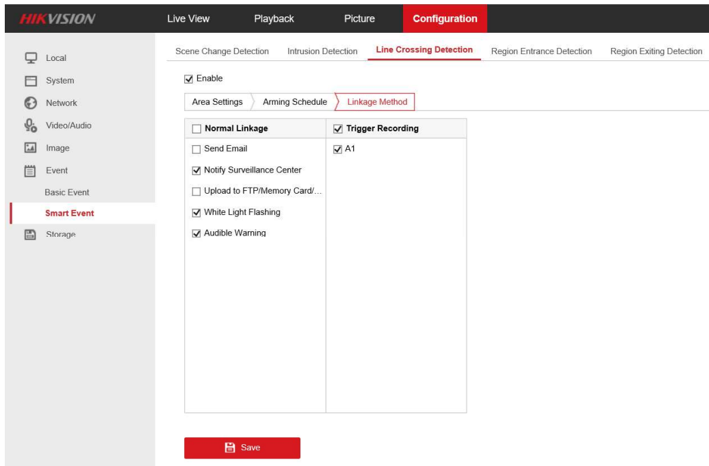
Figure 7 Linkage Method
