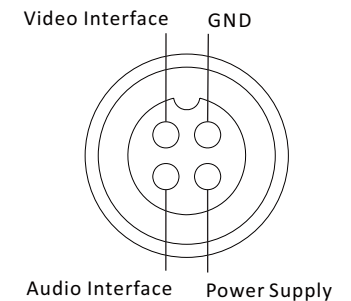
Figure 1-2 Cross Section of Aviation Plug
