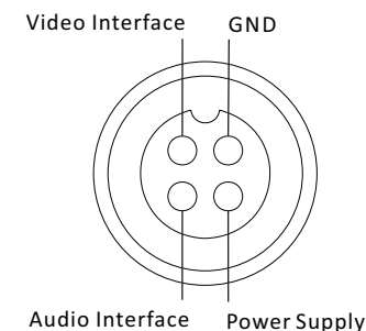
Figure 1-2 Cross Section of Aviation Plug
