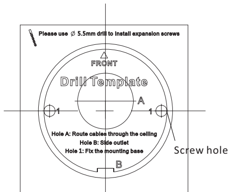
Figure 2-1 The Drill Template
