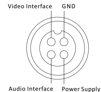
Figure 1-2 Cross Section of Aviation Plug
