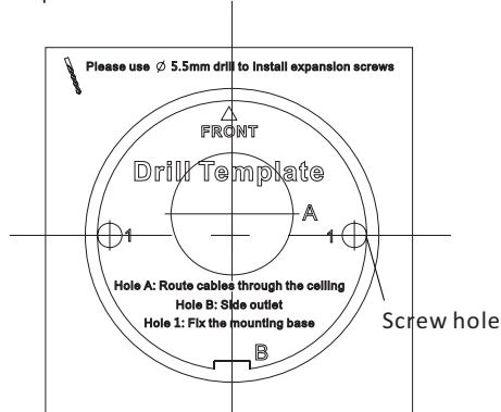
Figure 2-1 The Drill Template
