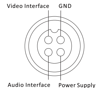
Figure 1-2 Cross Section of Aviation Plug
