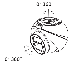
Figure 2-7 3-axis Adjustment
