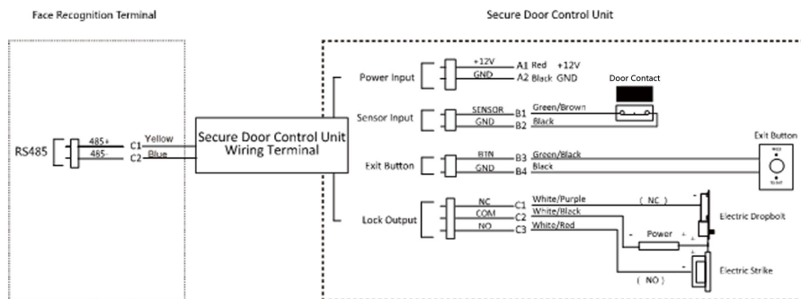
Figure 4-4 Secure Door Control Unit Wiring
