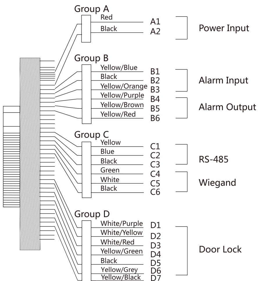
Figure 4-1 Terminal Diagram
