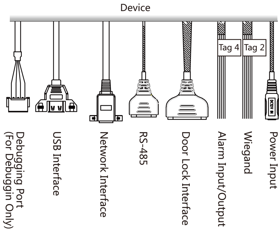
Figure 4-2 Wiring Interface
