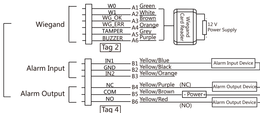
Figure 4-3 Device Wiring
