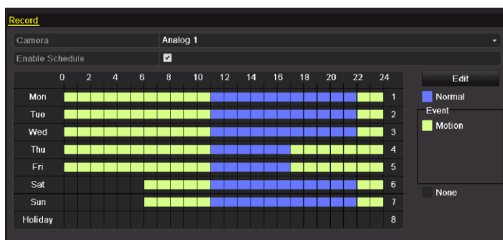
Figure 5.10 Etablir la programmation
