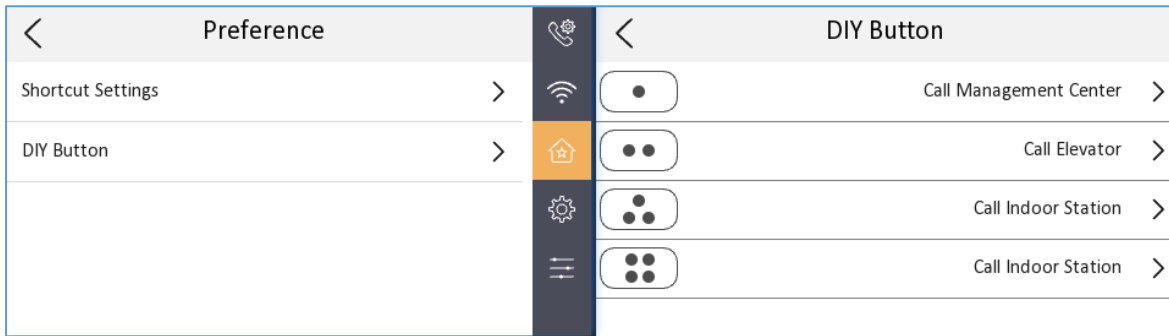
(local configuration interface of indoor station)
