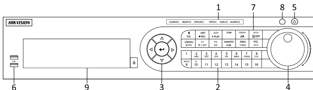
Figura 1–6 Panel frontal de las series DS-8100HQHI-F/N y DS-8100HUHI-F/N
