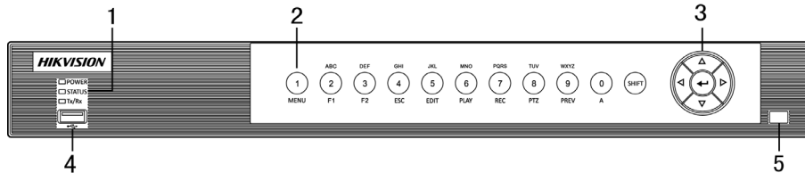
Figura 1-4 Panel frontal de las series DS-7200HUHI-F/N y DS-7600HUHI-F/N
