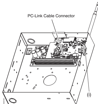
Figure 2 PC1616/1832/1864 Control Panel
