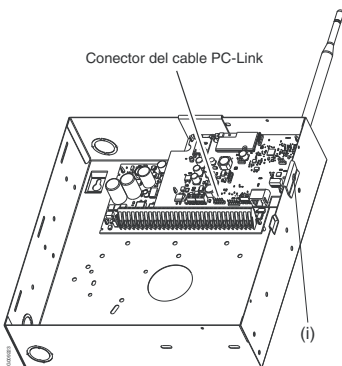
Figura 2 Panel de control PC1616/1832/1864
