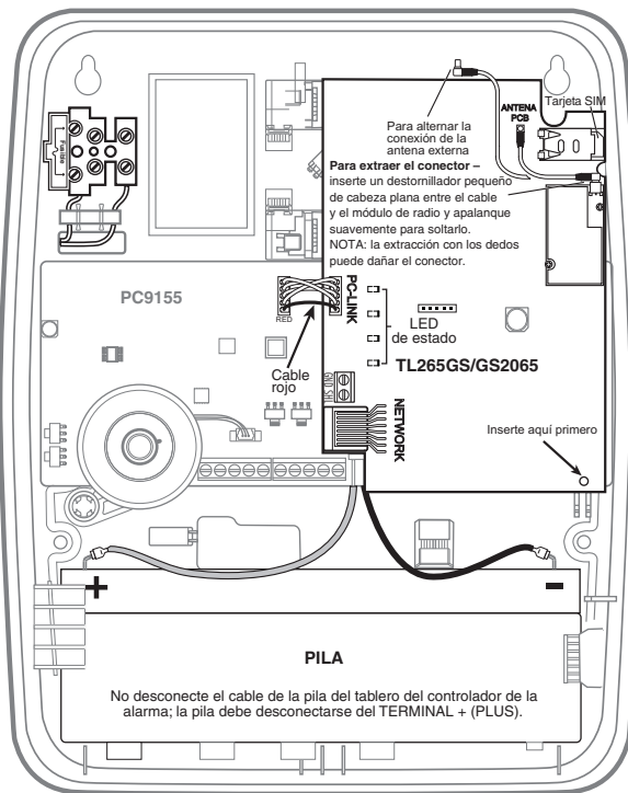
Figura 4 Panel de control PC 9155
